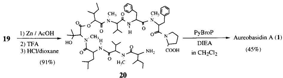
Scheme 5. Cyclization
