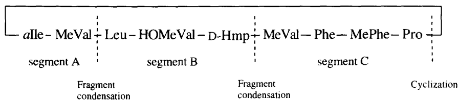
Fig. 2. Synthetic strategy
